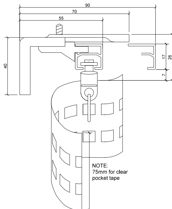
Series 50 Milan FACE FIX 40mm PROJECTION BRACKET No 7451
